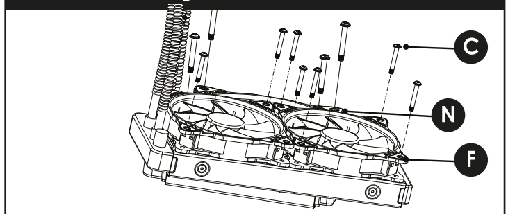
INTEL & AMD LIQUID COOLING HEATSINK INSTALLATION GUIDE
